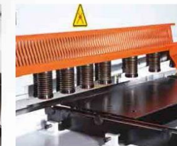
Collapsible finger protection. (standard) In order to control angled cuttings and drawn lines front part of protection can be pulled up by operator. (Switch protected)
